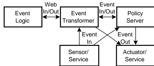
Fig. 3. Event Handling
